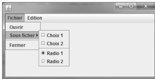
FIGURE 27.9 – Premier menu
